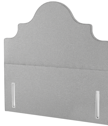
Mantle Deep
