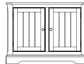
2 Door Sideboard (features internal drawer) H 875mm W 1165mm D 450mm
