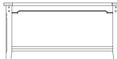
Coffee Table with Shelf H 490mm W 1000mm D 600mm
