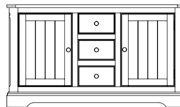
2 Door 3 Drawer Sideboard H 875mm W 1530mm D 450mm
