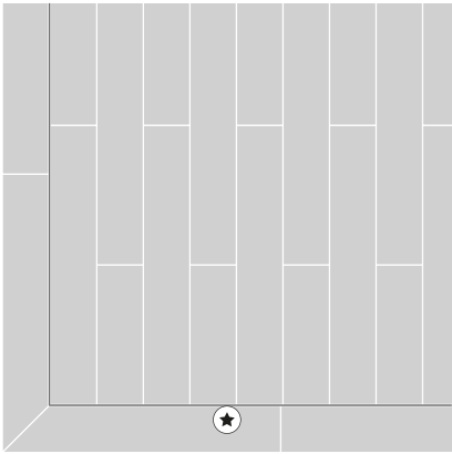
Full plank perimeter with inlay strip
